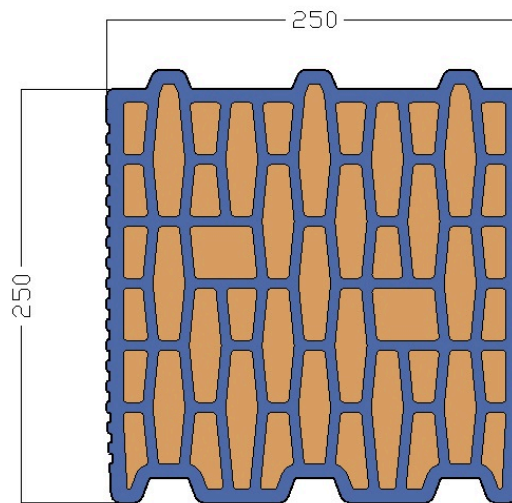
Figure 2. Cross section of the block
