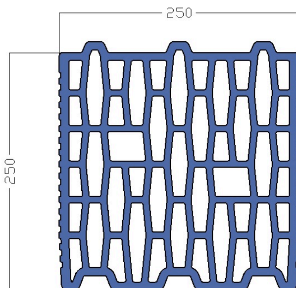
Figure 1. Geometry of the block
