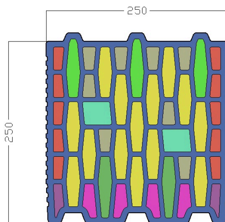
Figure 2. Cross section of the block and air voids
