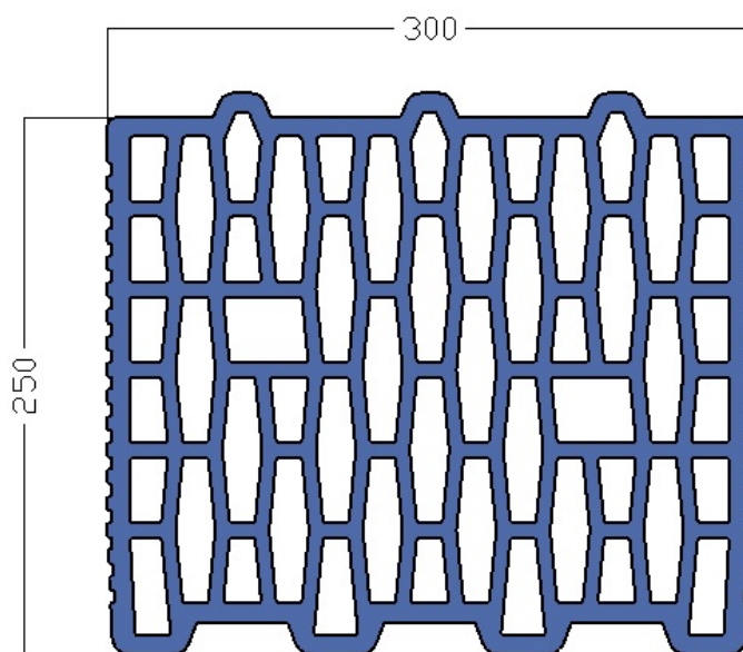
Figure 1. Geometry of the block
