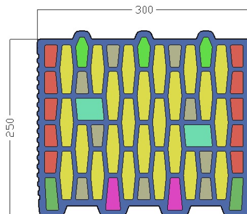
Figure 2. Cross section of the block and air voids
