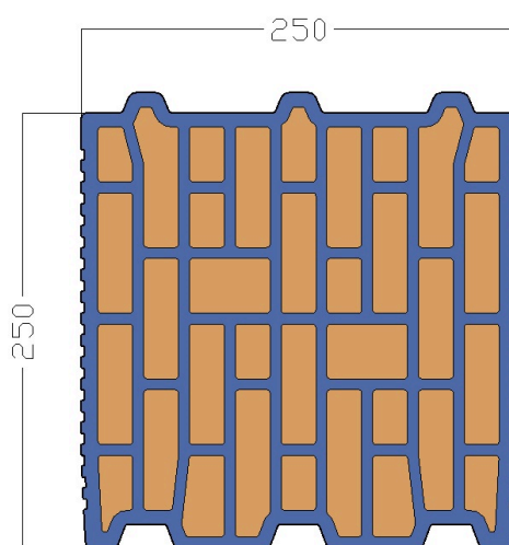
Figure 2. Cross section of the block
