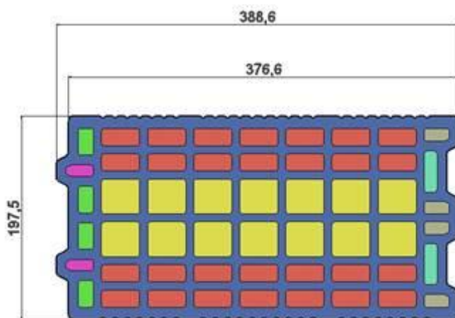
Figure 2. Cross section of the block and air voids
