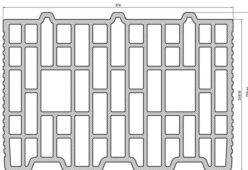
Figure 1. Geometry of the block
