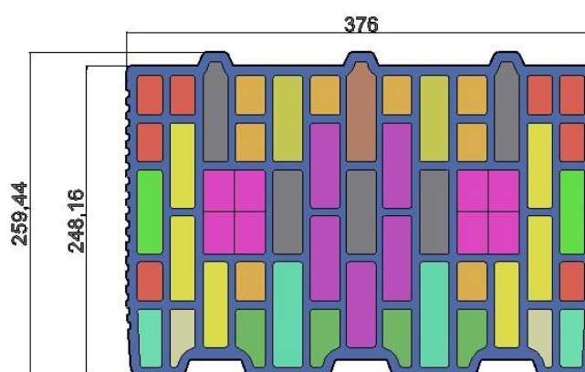
Figure 2. Cross section of the block and air voids
